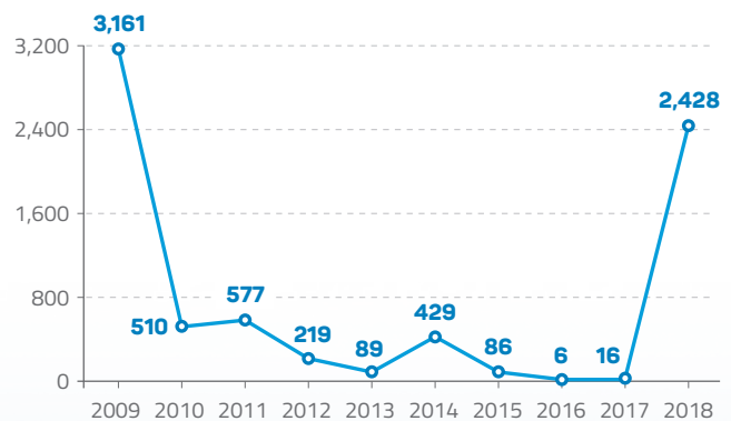
THE TREND OF GREATER FLAMINGO POPULATION IN LIBYA during the period from 2009-2018
